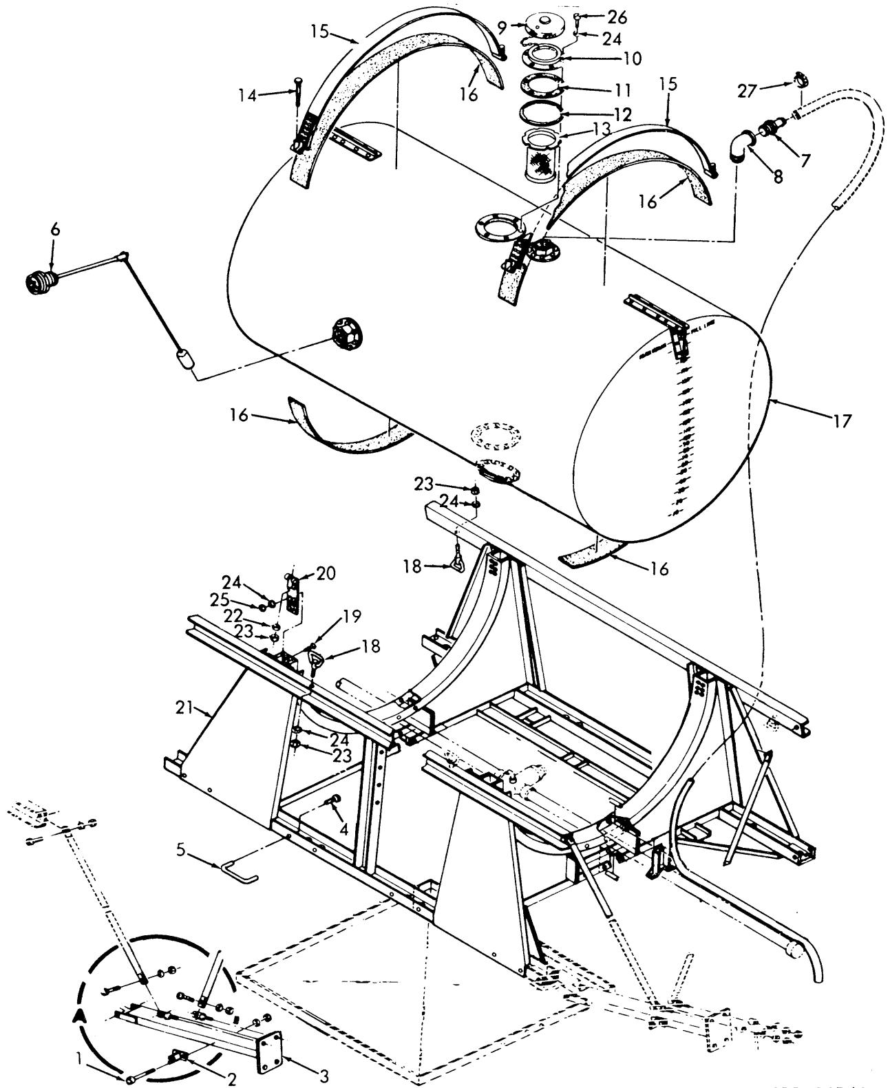
Figure 4. Sprayer Assembly, Tank and Related Parts
